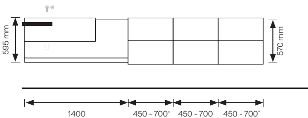
MI03 6 Standard-Laden
