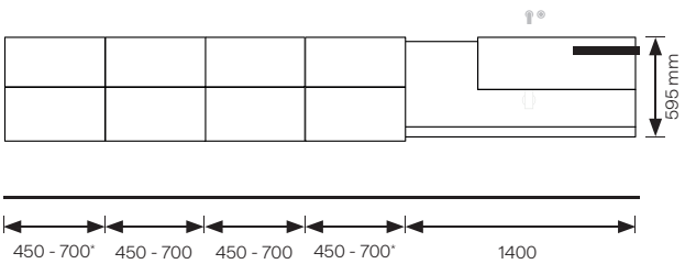
MI06 8 Standard-Laden
